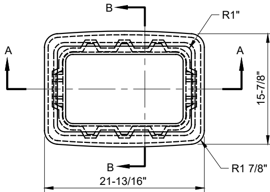
METER BOX TOP VIEW
